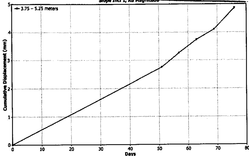
FIG. 5 Displacement Versus Time at Specific Depth Interval
