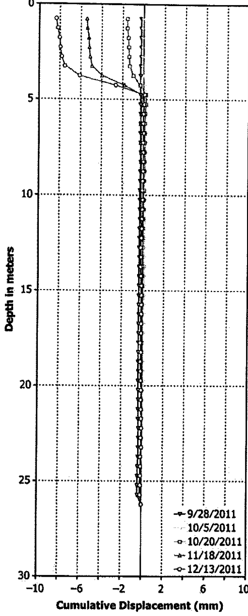
FIG. 4 Displacement Versus Depth and Time
