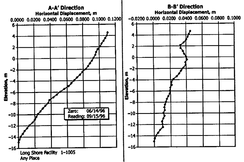
FIG. 3 Plot of Reduced Inclinometer Data
